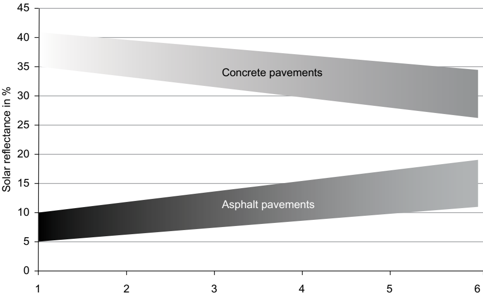
FIGURE 13: CHANGE IN SOLAR REFLECTANCE OF PAVEMENT TYPES, IN YEARS
