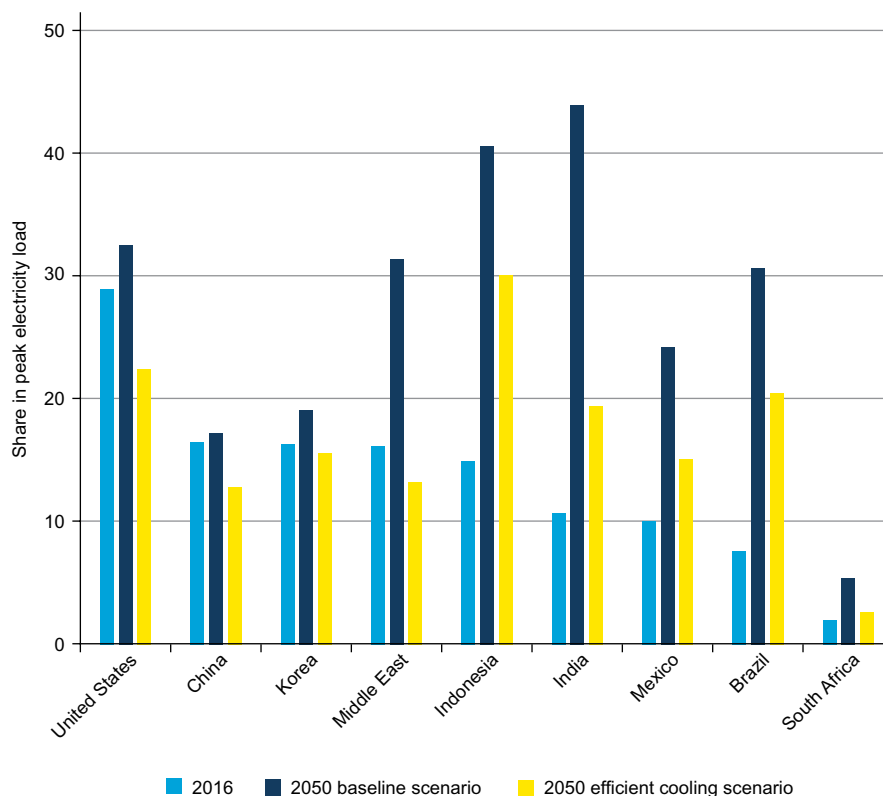
FIGURE 3: CONTRIBUTION OF SPACE COOLING TO PEAK ELECTRICITY DEMAND
