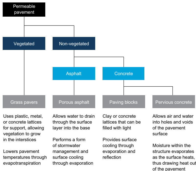
FIGURE 15: PERMEABLE PAVEMENT DESIGNS
