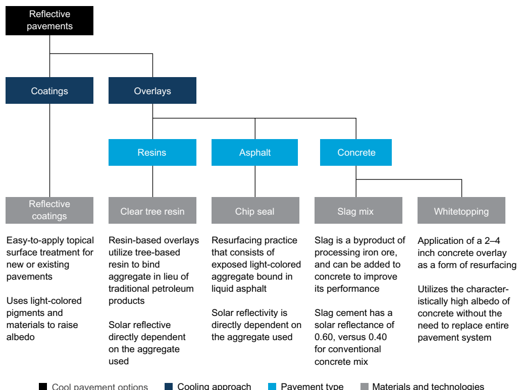
FIGURE 11: REFLECTIVE PAVEMENT PRODUCT OPTIONS
