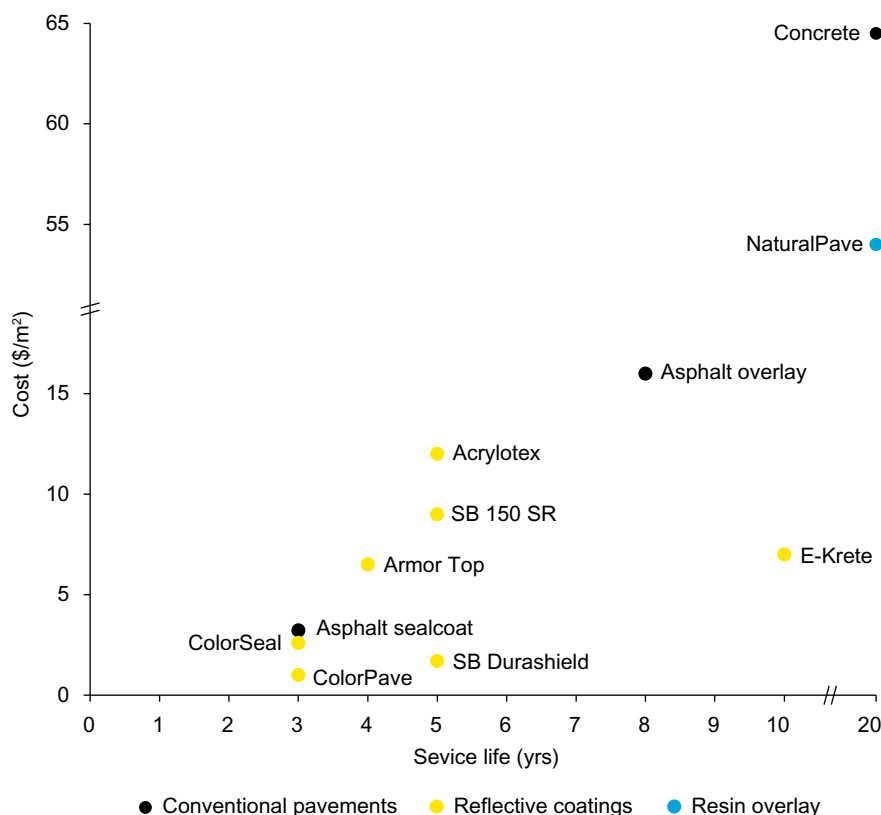
FIGURE 12: COOL PAVEMENT PRODUCT COST VERSUS SERVICE LIFE
